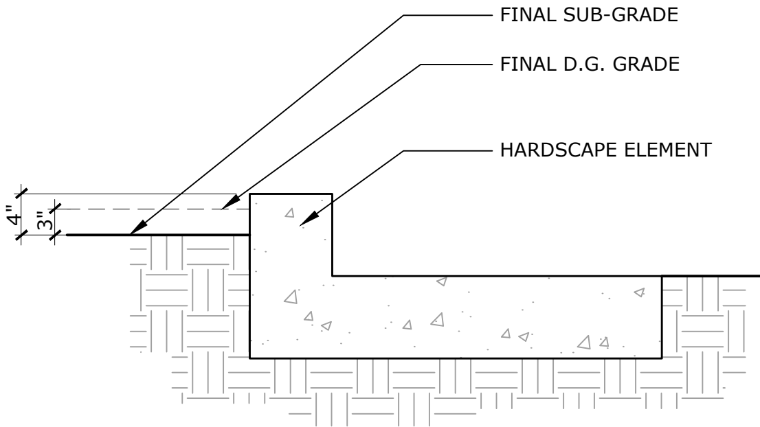
FINAL GRADE D.G. DETAIL
