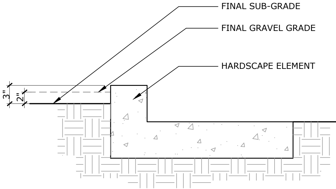
FINAL GRADE GRAVEL DETAIL
