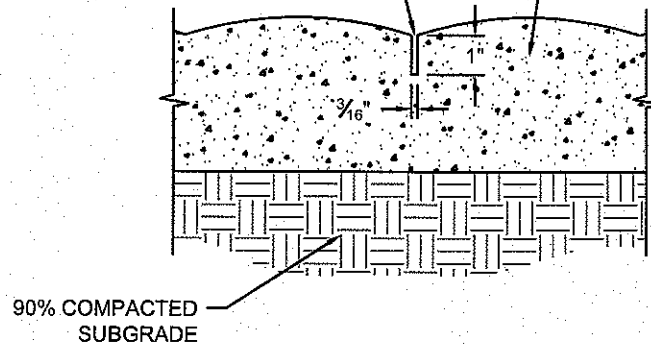
CONTROL JOINT
