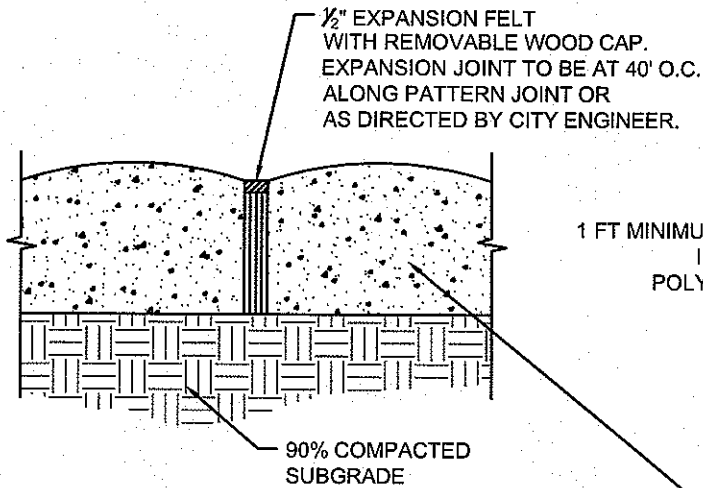
EXPANSION JOINT
