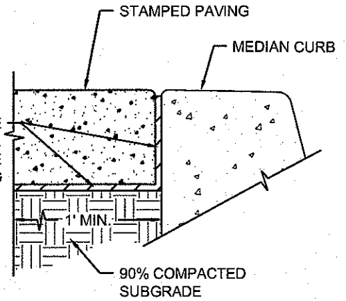
PAVING-CURB INTERFACE
