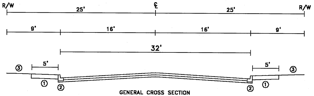
GENERAL CROSS SECTION
